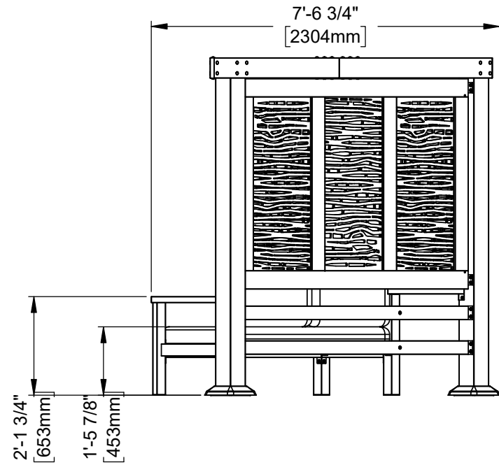
MODERN CABANA WITH FURNITURE FOOTPRINT
