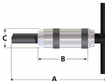
TYPE IV Non-Captive Prewinder
