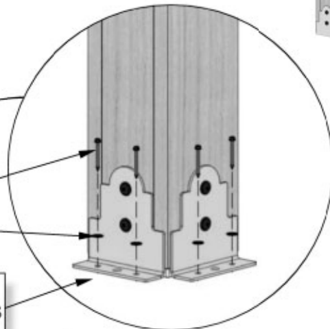
120 (x16) SCREW - 2" 630 (x16) WASHER - 8x19
