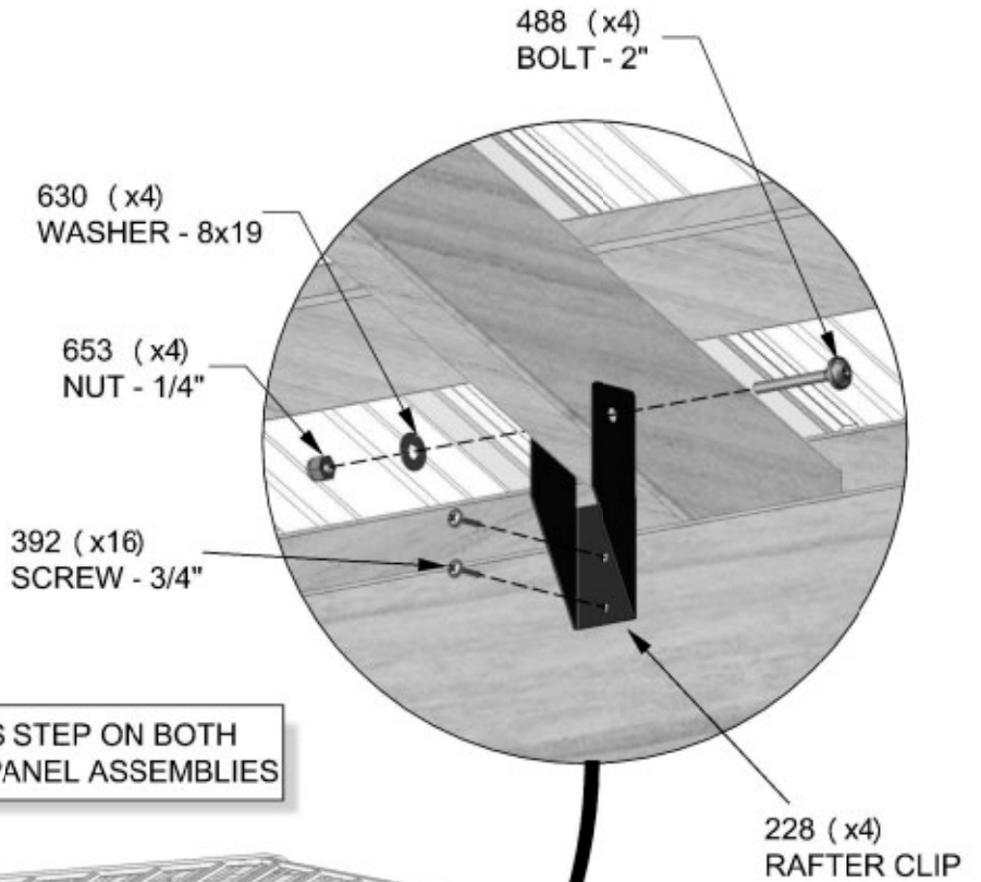
H100488 | BOLT WH BLK (8) | 1/4x2
